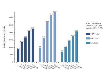
Cytometric bead array sample test of MP51585-1, ATG7 Monoclonal Matched Antibody Pair, PBS Only. Capture antibody: 67341-3-PBS. Detection antibody: 67341-4-PBS.
