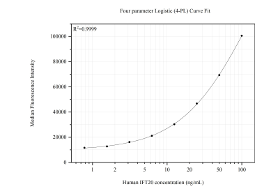
Cytometric bead array standard curve of MP51743-1, IFT20 Monoclonal Matched Antibody Pair, PBS Only. Capture antibody: 60765-2-PBS. Detection antibody: 60714-1-PBS. Standard:Ag4718. Range: 0.781-100 ng/mL
