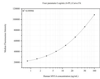
Cytometric bead array standard curve of MP51759-1, MYL6 Monoclonal Matched Antibody Pair, PBS Only. Capture antibody: 68142-1-PBS. Detection antibody: 68142-2-PBS. Standard: Ag13091. Range: 0.781-100 ng/mL.
