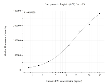
Cytometric bead array standard curve of MP51787-1, CPA1 Monoclonal Matched Antibody Pair, PBS Only. Capture antibody: 68826-2-PBS. Detection antibody: 68826-3-PBS. Standard:Ag8579. Range: 0.781-100 ng/mL.
