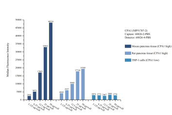
Cytometric bead array sample test of MP51787-2, CPA1 Monoclonal Matched Antibody Pair, PBS Only. Capture antibody: 68826-2-PBS. Detection antibody: 68826-4-PBS.
