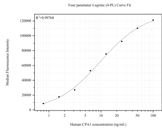
Cytometric bead array standard curve of MP51787-2, CPA1 Monoclonal Matched Antibody Pair, PBS Only. Capture antibody: 68826-2-PBS. Detection antibody: 68826-4-PBS. Standard:Ag8579. Range: 0.781-100 ng/mL
